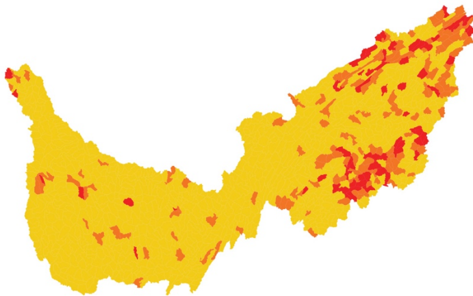
Figure 4: Threat of forest insects and disease.
