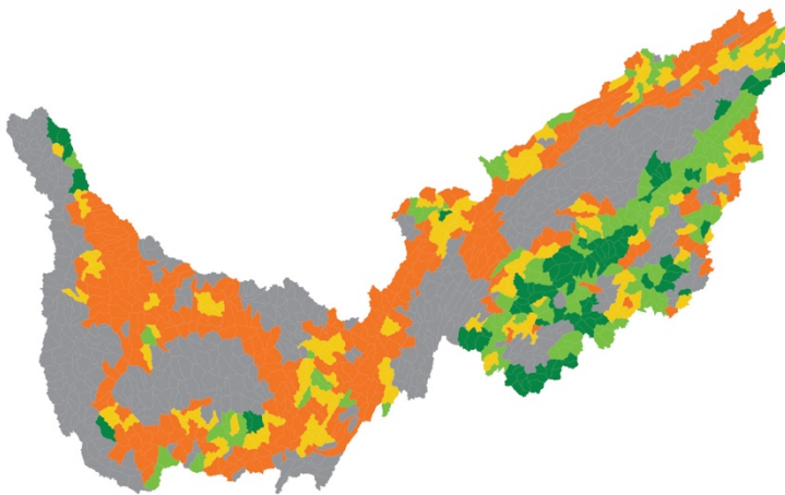
Figure 12: Evaluation of protected land status within connected forests in the TRB.
