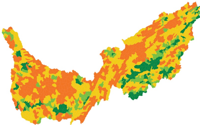
Figure 13: Percent wetlands protected from development.
