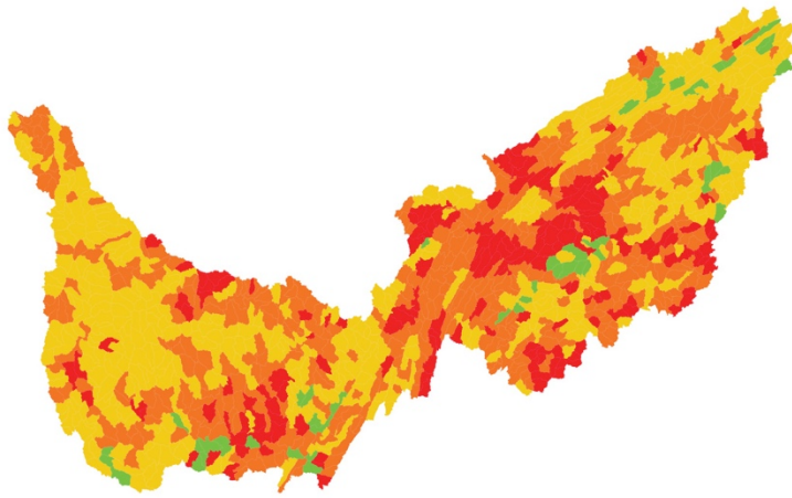
Figure 1: Development threat in forests throughout the TRB.
