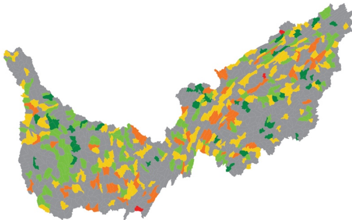
Figure 8: The Index of Biotic Integrity (IBI) based on TVA sampling campaigns between 2010 and 2014.
