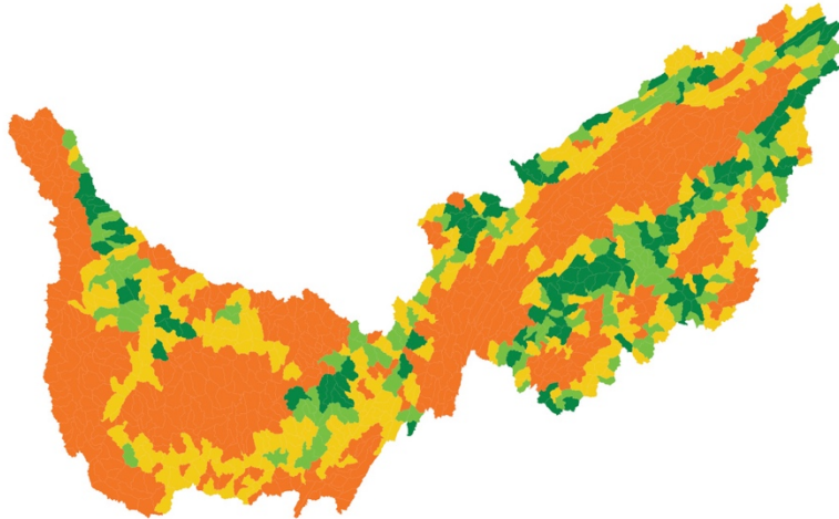
Figure 6: Connected forest area.
