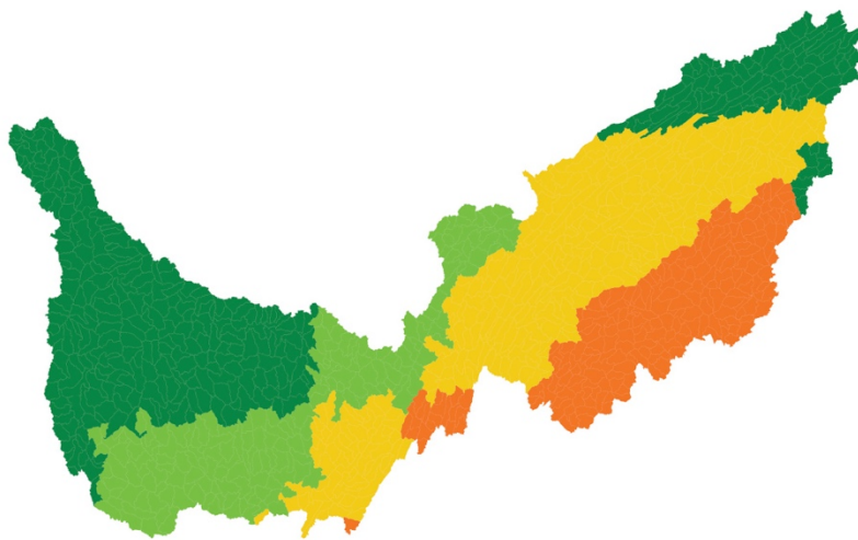
Figure 2: Months of extreme drought, evaluated via the Palmer Drought Severity Index, over the past 10 years.
