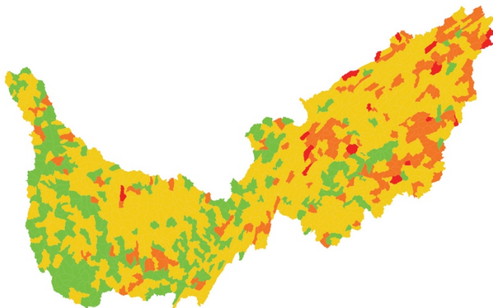
Figure 7: Aquatic connectivity scores that reflect data on both dam and road crossing density.
