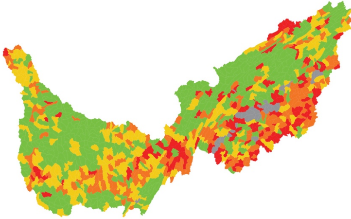
Figure 10: The percentage of treated high priority cropland.
