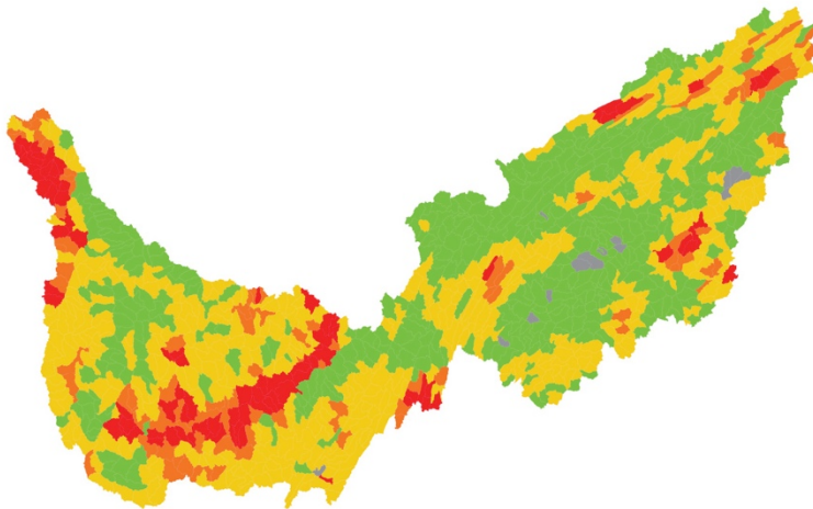
Figure 5: The area of croplands in priority 1 risk for runoff, as assessed by the Soil Vulnerability Index.
