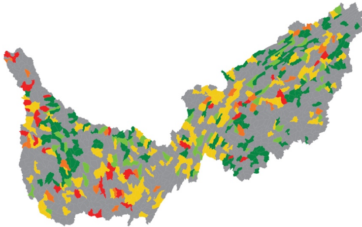
Figure 9: Ephemeroptera , Plecoptera and Trichoptera scores
