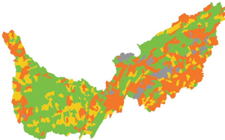
Figure 11: The percentage of high priority area that has been treated for leaching.
